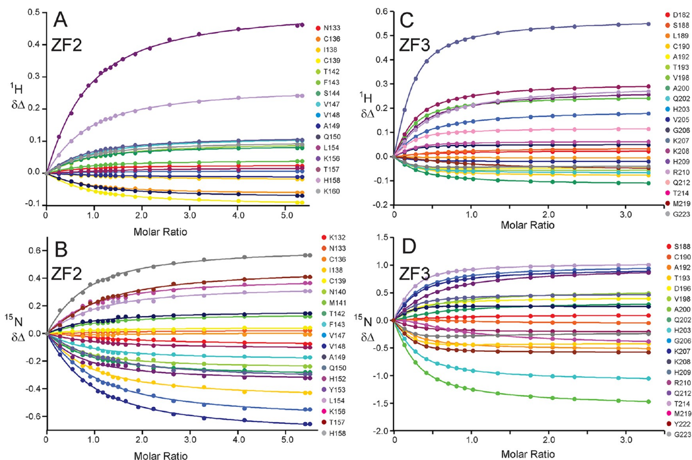
Figure 5. Chemical-shift perturbations for all measurable amide resonances upon binding VAImin RNA (derived from the data of Figure 3) plotted as a function of the molar ratio of [RNA]/[ZF]. Experimental data are represented by filled circles; lines of corresponding colors show the results obtained from global fits of all of the ^1\text{H} and ^{15}\text{N} \Delta\delta data for a given titration to a two-site binding model using the program nmrKd2 . 23 (A) ^1\text{H} data for the ZF2/VAImin RNA titration. (B) ^{15}\text{N} data for the ZF2/VAImin titration. (C) ^1\text{H} data for the ZF3/VAImin titration. (D) ^{15}\text{N} data for the ZF3/VAImin titration.
